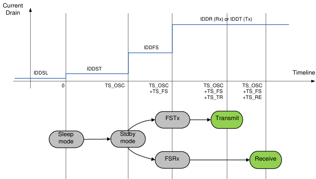
Figure 17. Startup Process
