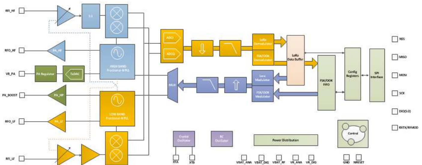
Figure 3. RF96/97/98 Block Schematic Diagram
